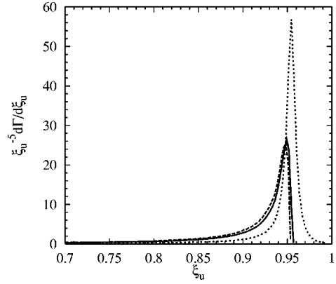
FIG. 4. The weighted \xi_u spectrum without (dotted curve) and with (solid curve: \alpha_s=0.2 ; dashed curve: \alpha_s=0.27 ) the QCD radiative correction. The four parameters for the distribution function are taken to be \alpha=\beta=1 , a=0.9548 , and b=0.005444 . All the spectra are normalized to have unit area.
