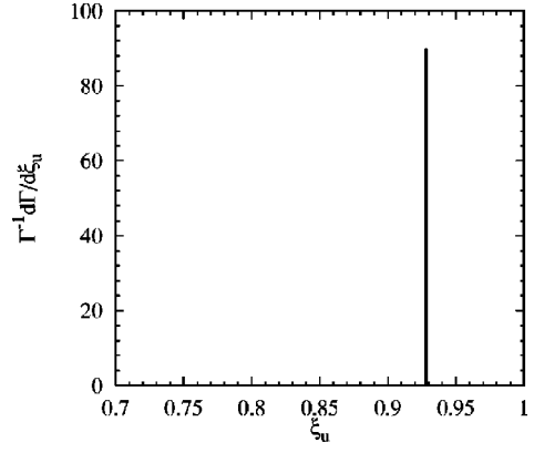
FIG. 1. The \xi_u spectrum in the tree level and virtual gluon exchange processes b \rightarrow ul\nu . The b -quark mass m_b = 4.9 GeV is used.
